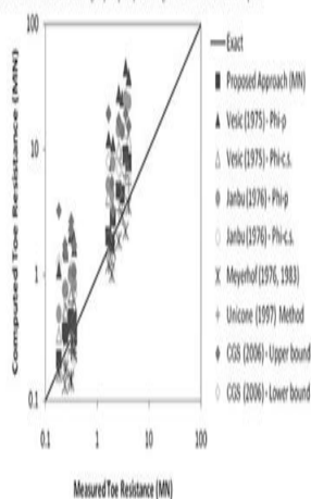
Fig. 18. Computed versus measured end-bearing capacity of piles using different methods on one plot.
